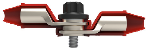
The Lugsulation® Smart is stackable by design and parallel installation is possible
