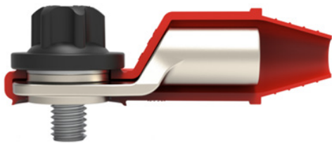
The Lugsulation® Smart is the ideal fit for flat contact surface terminals
